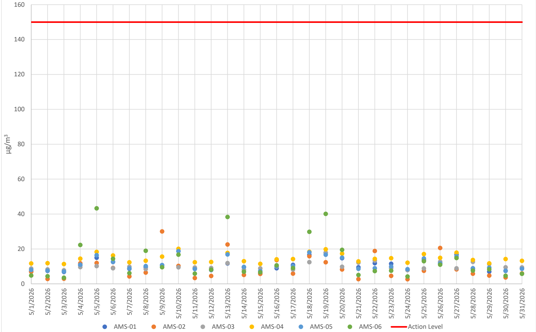
Figure 2.a - Dust Concentration 24-Hour Averages Industrial Campus May 1, 2026 – May 31, 2026 The Bellwether District
