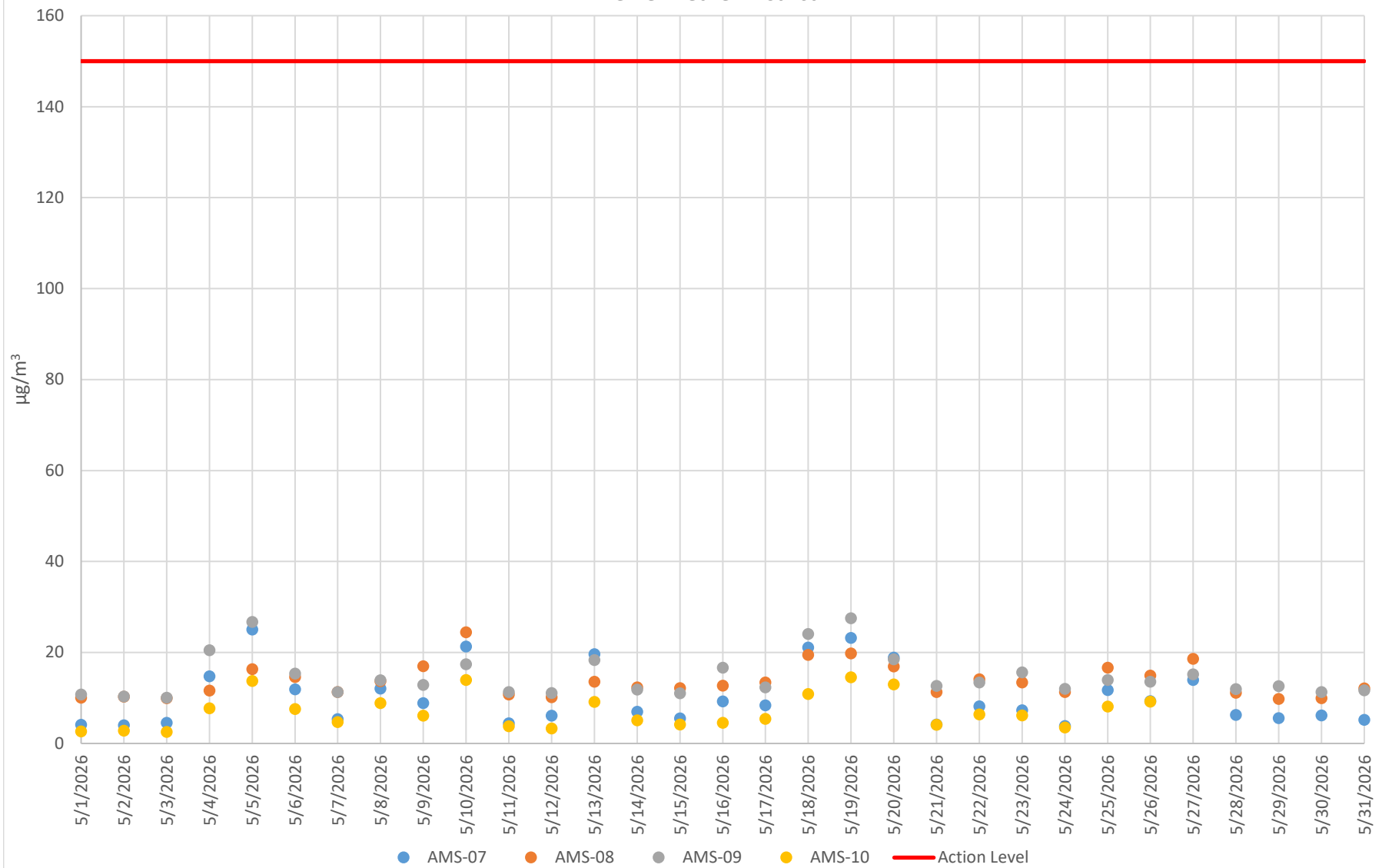
Figure 2.b - Dust Concentration 24-Hour Averages Innovation Campus May 1, 2026 – May 31, 2026 The Bellwether District
