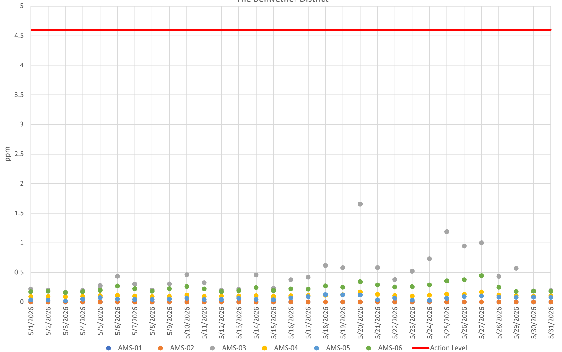
Figure 3.a - VOC Concentration 8-Hour Averages Industrial Campus May 1, 2026 – May 31, 2026 The Bellwether District
