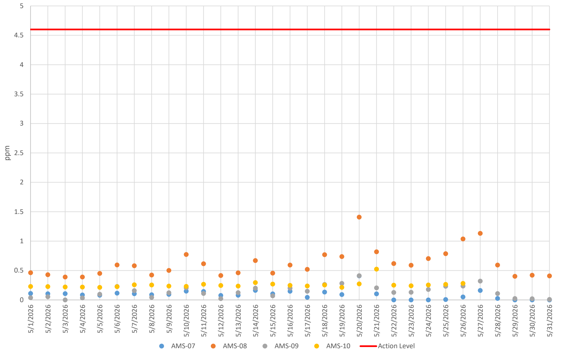
Figure 3.b - VOC Concentration 8-Hour Averages Innovation Campus May 1, 2026 – May 31, 2026 The Bellwether District
